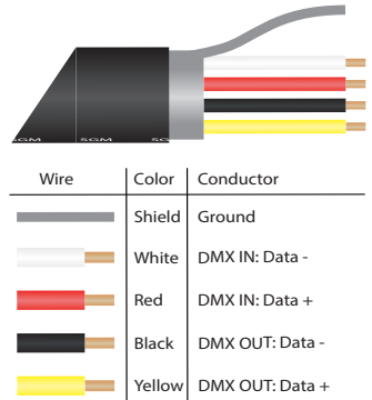
Figure 2: POI DMX Cable
