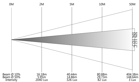
Lux Diagram
